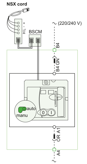
Communicating motor mechanism (MTC)
